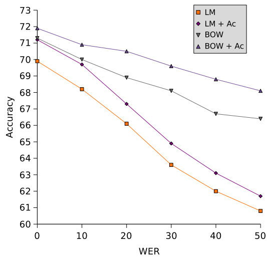
Fig. 1. Variation of question classification accuracy vs. WER
