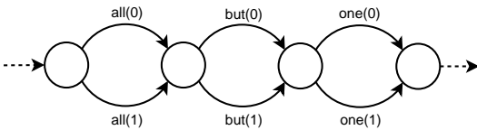
Fig. 1. Word graph with prosodic variants
