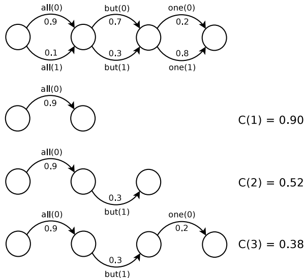
Fig. 2. Obtaining n-gram counts from lattice chunks
