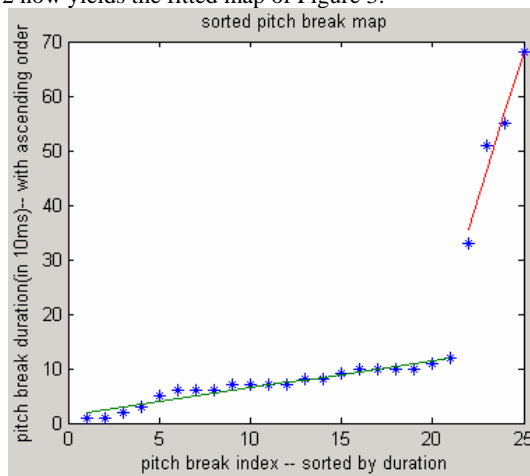
Figure 3: Linear fold algorithm
