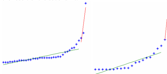
Figure 4: Illustrating the two pass linear fold algorithm: result of the first pass is to the left and the second pass to the right.
