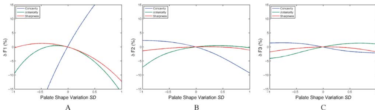
Figure 6. The acoustic impact of varying palate shape in tubes of nonuniform width, averaged across subjects, corresponding to the articulation of a high-front vowel from the five speakers in this study. Palates were varied according to the three major modes of variation: concavity, anteriority, and sharpness. Change in frequencies of the first three formants are plotted as a function of variation along these three modes. Palate shape changes are represented in terms of the SDs .
