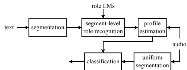
Figure 1: Linguistically-aided speaker diarization using role information.
