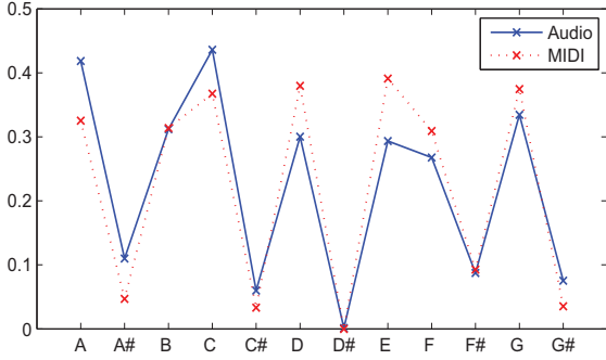
Fig. 2. An example of usage of pitch classes information; a comparison between music fingerprints from audio signal and MIDI data (BWV 772).
