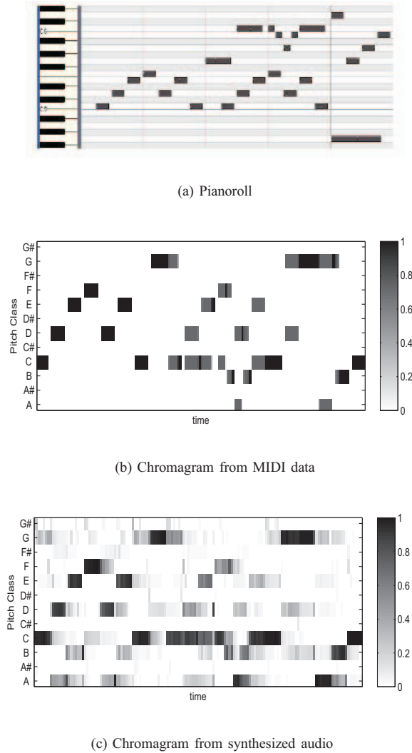
Fig. 1. An example of chromagram from MIDI data and synthesized audio signal compared with pianoroll (BWV772). The representation from audio is noisier compared with that obtained from MIDI.
