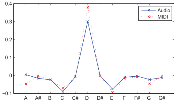
Fig. 3. An example of harmony structure information; a comparison between music fingerprints from audio signal and MIDI data (BWV 772).
