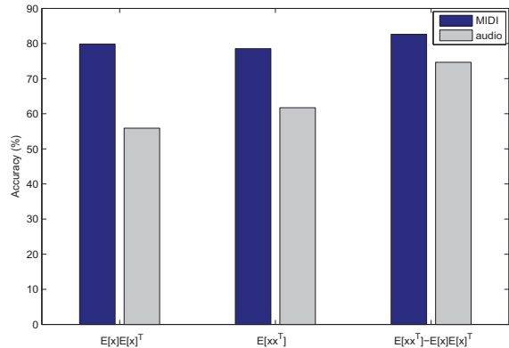
Fig. 4. Performance comparison between various second-order statistics using MIDI data and audio signal.
