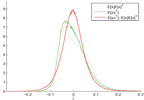
Fig. 5. Distribution of noise in similarity measure.
