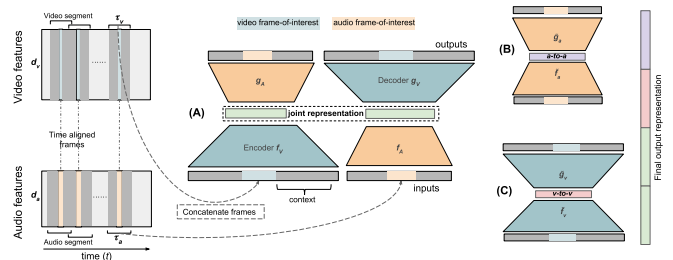
Figure 1: Schematic diagram of segment-level autoencoders for (A) joint representation (B) audio: a-to-a , and (C) video: v-to-v . Input video and audio features of dimensions d_v, d_a for an ad of duration t . Video and audio segments of length \tau_v, \tau_a
