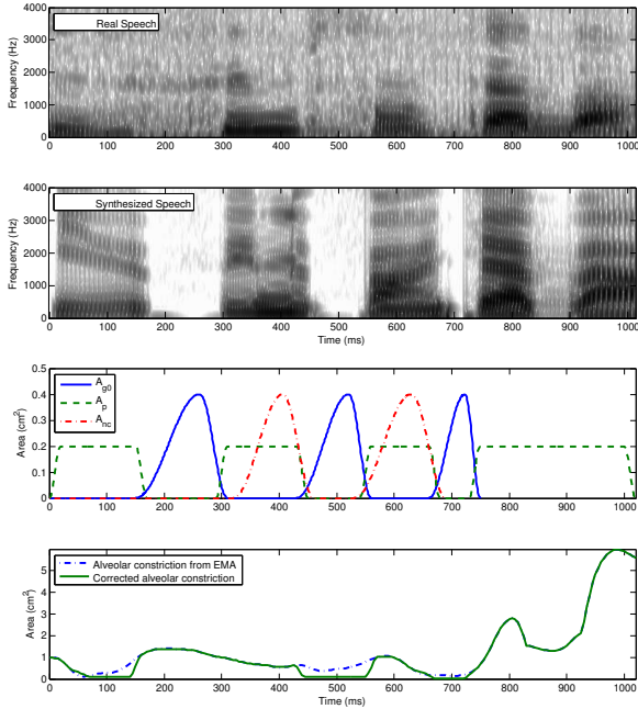
Figure 5: Synthesis results and (subset of) inputs for the utterance Il fume son tabac. Top to bottom: (i) spectrogram of recorded speech – note that audio is noisy; (ii) spectrogram of synthesized speech; (iii) slow-varying component of glottal area A_{g0} ; amplitude A_p of fast-varying component of glottal area; area of velopharyngeal port A_{nc} (iv) cross-section area at the alveolar ridge (16th out of 17 cross-sections, numbered from glottis).
