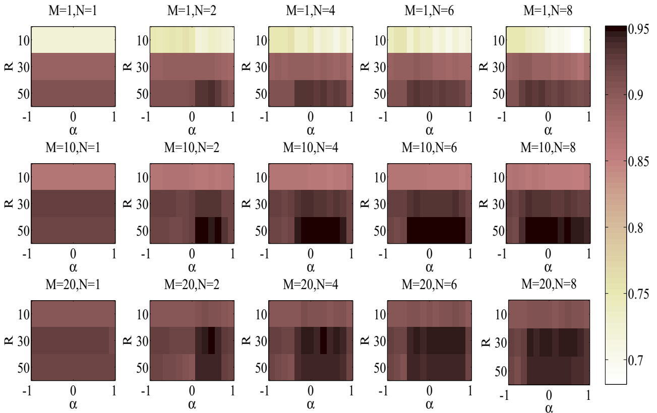
Figure 1: This figure shows the VAD frame accuracy for the development set of channel A for various parameters of the multi-band LTSV. R represents the analysis window length, M the frequency smoothing, \alpha the warping factor and N the number of filters. The bar on the right represents the frame accuracy. This figure indicates that for channel A increasing the number of bands ( N ) improves the accuracy. Also, indicates that smoothing ( M \geq 100 ) and analysis window ( R ) are crucial parameters for the multi-band LTSV as observed in the original LTSV [11].
