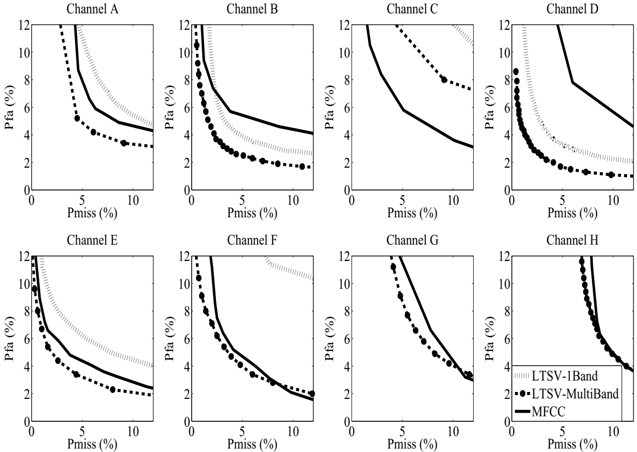
Figure 2: This figure shows the ROC curve of Pfa vs Pmiss for channels A-H of the multi-Band LTSV (LTSV-MultiBand) and the two baselines (1-band LTSV and MFCC). For channels G and H the 1-band LTSV ROCs are out of the boundaries of the plots, hence they do not appear in the figure. The same legend applies to all subfigures.
